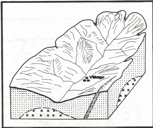
Fig:1 Generalised diagram of a Drainage Basin
