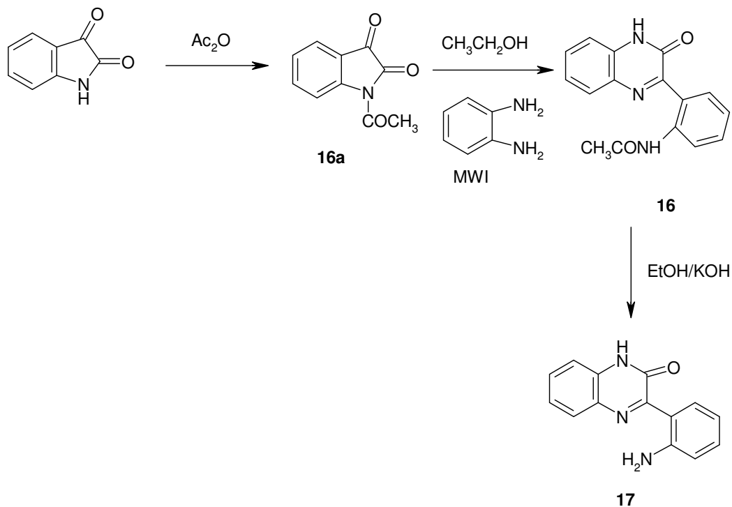
Figure 4. Synthesis route to 2-quinoxalinones 16 and 17 .
