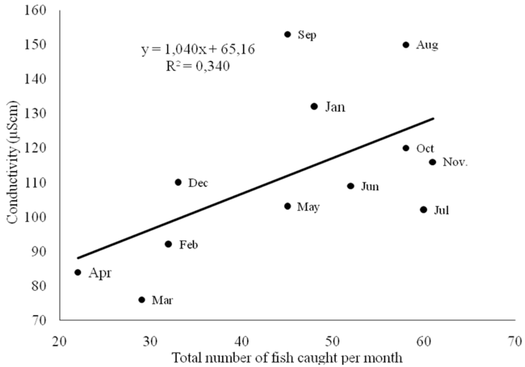
Figure 1: Variation in conductivity ( \mu\text{Scm} ) against total number of fish caught per month.
