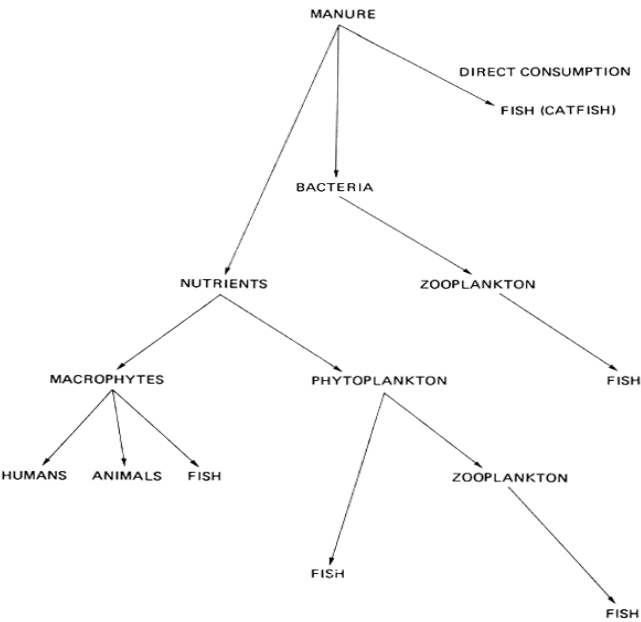
Figure 1: Manure-fish recycling.
